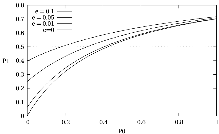
Figure 3. The effect of phoneme mutual confusability on the spread of the merger. Note that even when perception error rate is zero, there still needn’t be a majority of M_+ speakers for the merger to spread; the critical value here is 0.43.
