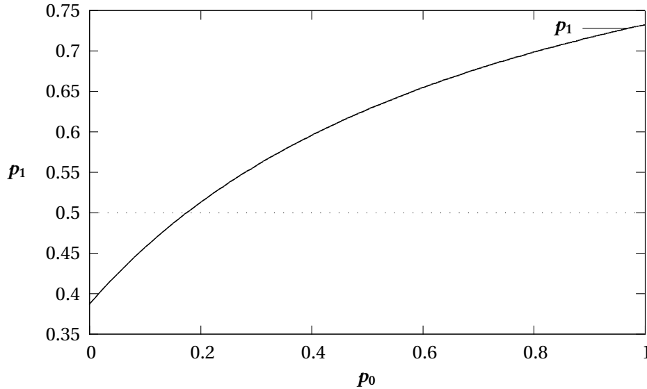
Figure 2. The dynamics of learning from p_0 to p_1 for the cot-caught merger. The critical threshold for p_0 , which is 0.168, is obtained when p_1 \geq 1/2 .
