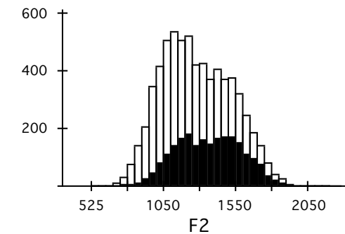
Figure 12.5. Distribution of /ow/ tokens not before /l/ for all of North America (N = 6736). Black = vowels with coronal onsets (N = 2251).
