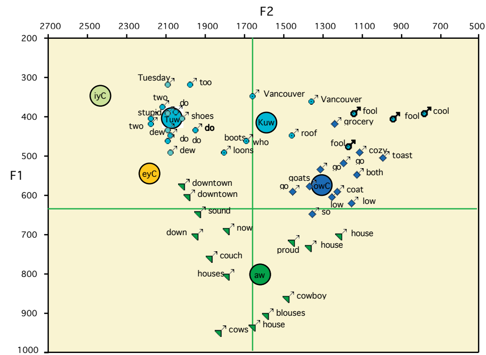
Figure 12.9. Canadian pattern of /Tuw/ fronting in vowel system of Lena M., 34, Toronto, ON, TS 645. Vowels before /l/ highlighted
