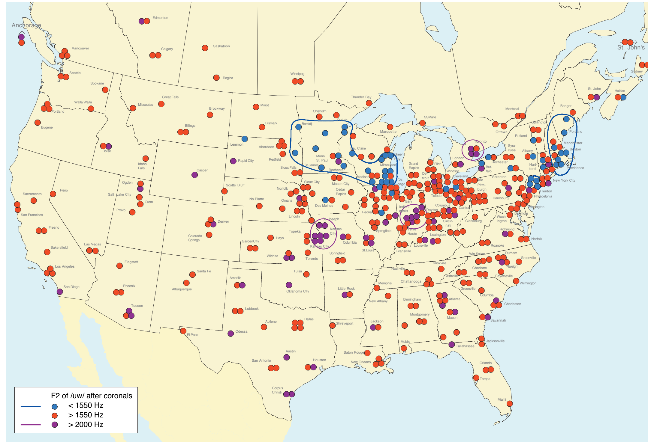
Map 12.1. Fronting of /uw/ after coronals (Tuw)
