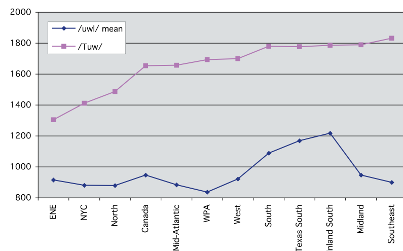
Figure 12.7. Second formant of /Tuw/ and /uw/ before /l/ by Region. Inland South and Texas South separated from other regions of the South
