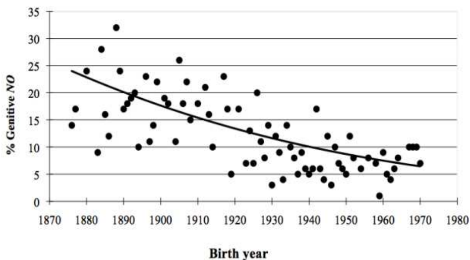
Figure 1: Scatterplot of the rate of no in the MJD corpus (Nambu and Matsuda 2007)
